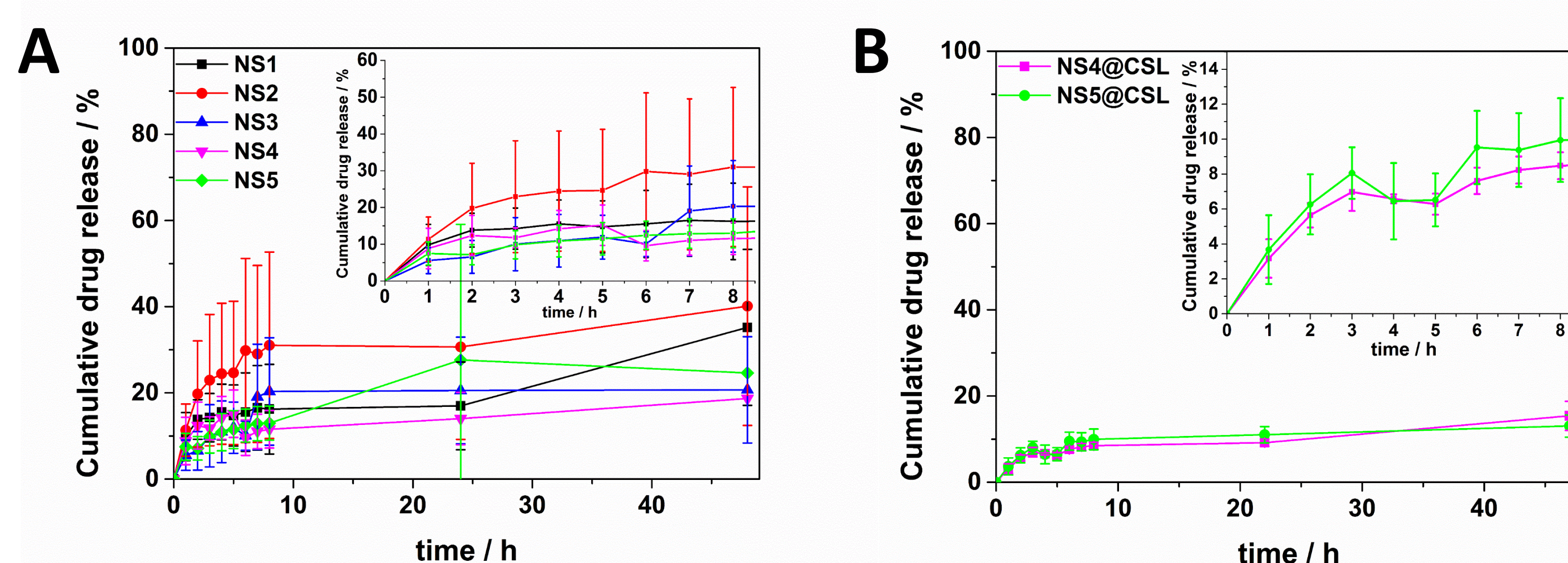
Fig. 2. Cumulative drug release profiles for core (A) and core/shell (B) beads loaded with ciprofloxacin.
