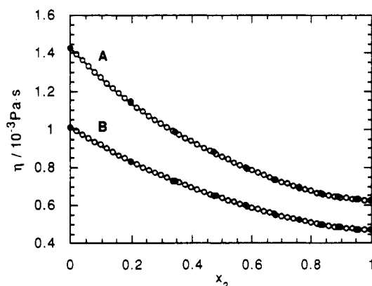
Figure 1. Variation of viscosity \eta for dioxane (1) + methanol (2): ●, experimental values; ○, values calculated from eq 9; (A) 15 °C; (B) 35 °C.
